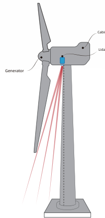
Threshold detection
