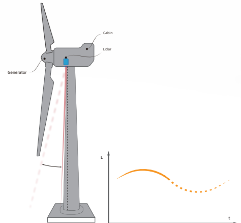
Trend detection
